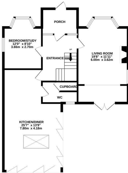
GROUND FLOOR 792 sq.ft. (73.5 sq.m.) approx.
